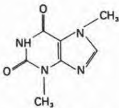
THEOBROMINE
